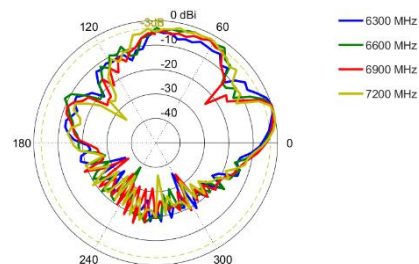
Elevation: 6300 – 7200 MHz
