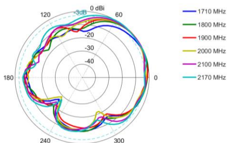
Elevation: 1710 – 2170 MHz
