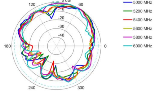
Elevation: 5000 – 6000 MHz
